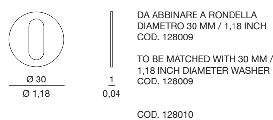
C. BOCCHETTA TONDA SLIM FORO CHIAVE DIAMETRO 30 MM - 1,18 INCH ROUND SLIM KEY HOLE ESCUTCHEON DIAMETER 30 MM - 1,18 INCH
