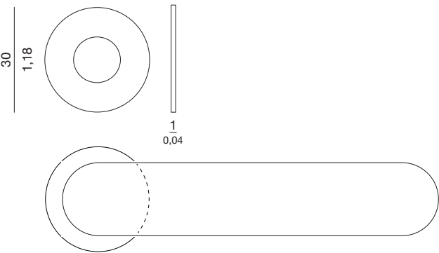
H. RONDELLA DIAMETRO 30 MM - 1,18 INCH 30 MM - 1,18 INCH DIAMETER WASHER
