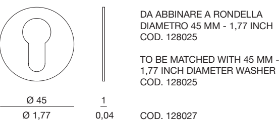
E. BOCCHETTA TONDA SLIM FORO CILINDRO DIAMETRO 45 MM - 1,77 INCH ROUND SLIM CYLINDER HOLE ESCUTCHEON DIAMETER 45 MM - 1,77 INCH
