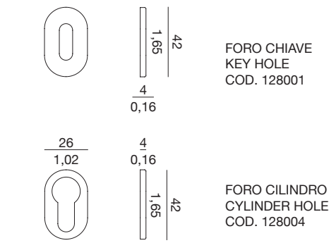
B. BOCCHETTA STANDARD / STANDARD ESCUTCHEON
