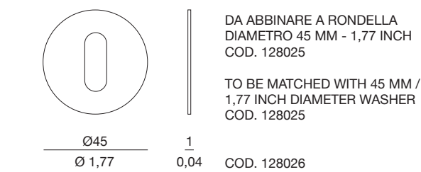
D. BOCCHETTA TONDA SLIM FORO CHIAVE DIAMETRO 45 MM - 1,77 INCH ROUND SLIM KEY HOLE ESCUTCHEON DIAMETER 45 MM - 1,77 INCH
